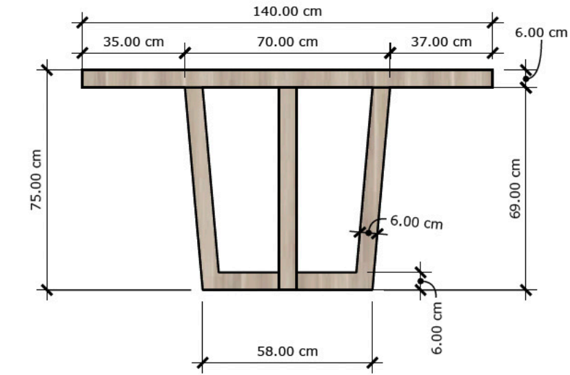
VISTA FRONTAL
