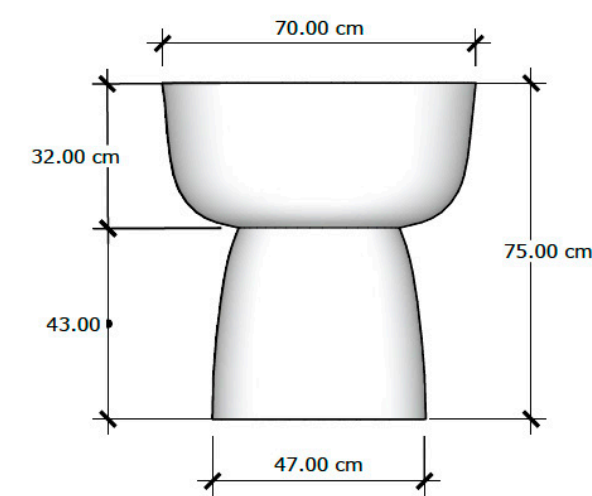
VISTA FRONTAL
